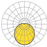
PGPC/1500 LED 7100 lm 840 \eta_{LB} 100 % lm/W 144 Direct/indirect 92/8 % UGR lat./long. 25.8/23.7
