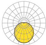
PGPC/1200 LED 4100 lm 840 \eta_{LB} 100 % lm/W 150 Direct/indirect 92/8 % UGR lat./long. 24.8/22.7
